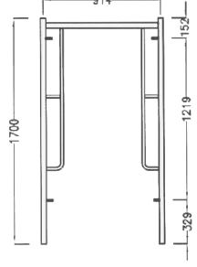
HT 103 Vertical Frame
