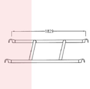
HT 201, 202, 203 Walking Frame
