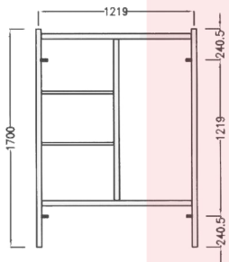
HT 107 Ladder Type Frame
