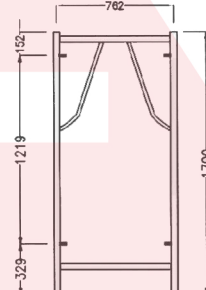
HT 105 Vertical Frame
