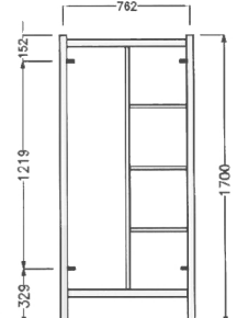
HT 106 Vertical Frame
