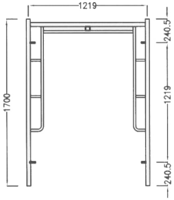
HT 101 Vertical Frame
