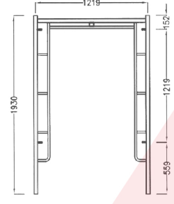
HT 101A Vertical Frame
