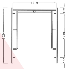
HT 102 Vertical Frame
