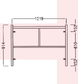
HT 109Ht Adjusting Frame
